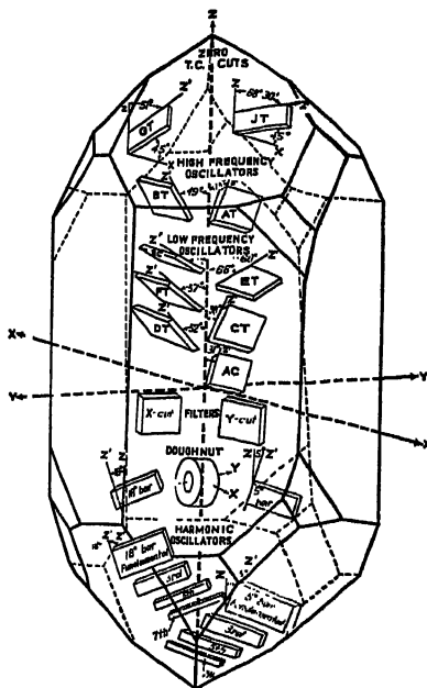
Standard types of cuts made in quartz crystals. The angle of the cut with respect to the natural faces of the crystal determines the electrical characteristics of the finished crystal plate.
